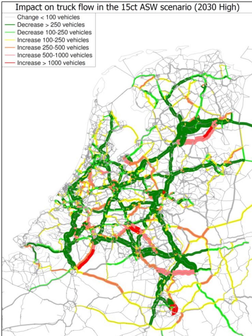
Figure 2: Impact on truck flow on the Dutch road network in the 15ct ASW scenario (2030 High)
