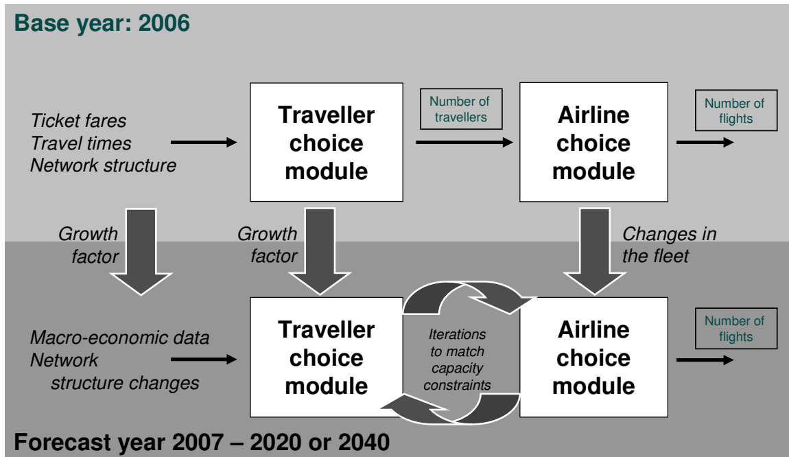
Figure 6 Structure of the AEOLUS model
